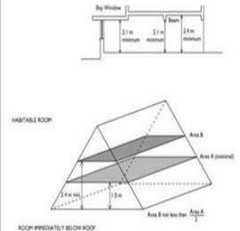
Diagram 3: Suggested height of habitable rooms
